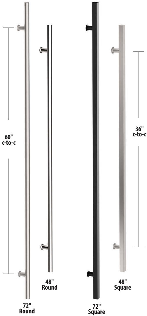
Standard Mounting
