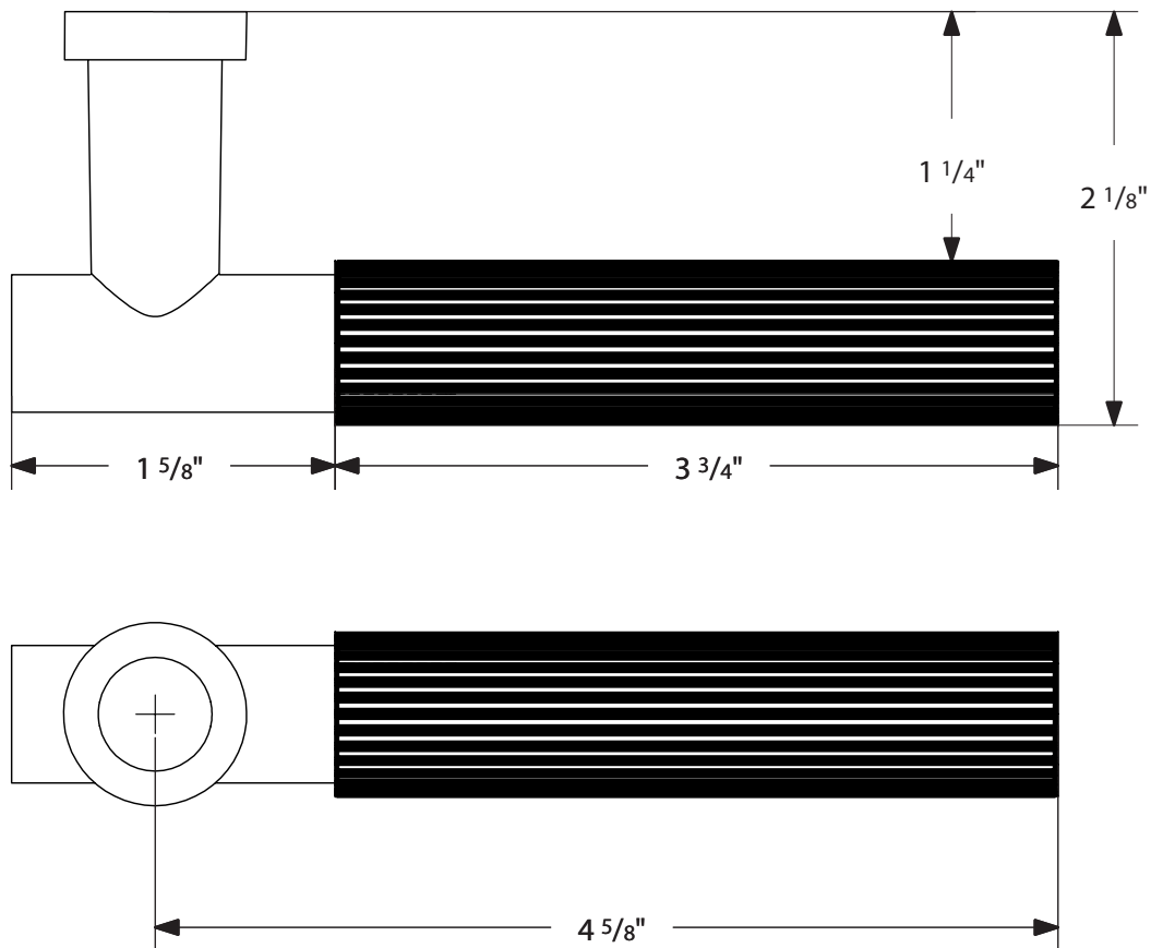
Straight Knurled Handle with T-Bar Stem
